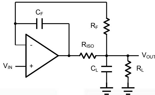
Figure 4. Indirectly Driving a Capacitive Load with DC Accuracy
