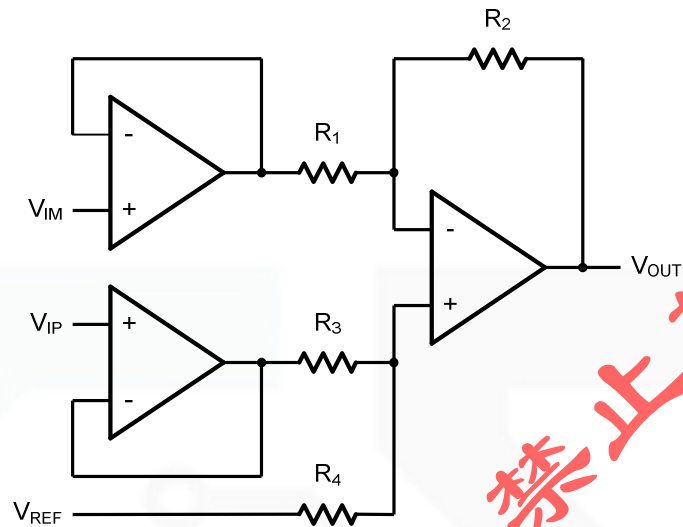
Figure 7. Instrument Amplifier
